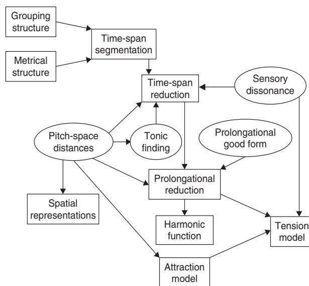
FIGURE 8. Flowchart of the components of the GTTM/TPS theory.
