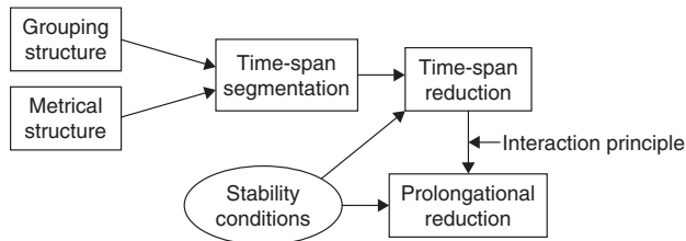
FIGURE 6. Flowchart of the components of the GTTM theory. (Subsidiary feedback arrows are not shown.)
